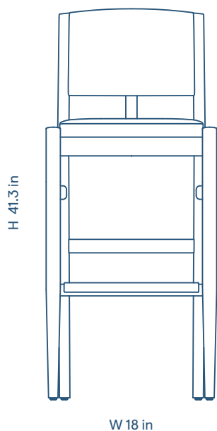
Front Elevation
