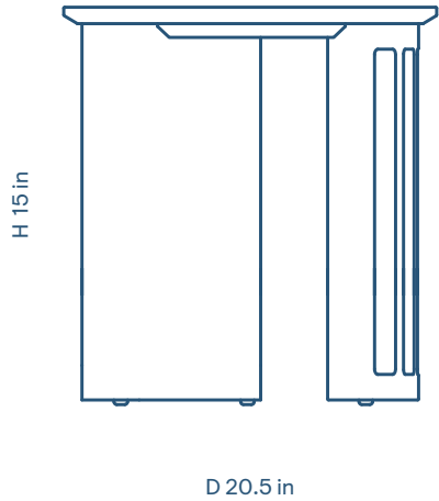
Side Elevation
